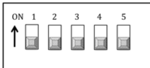
Five Position Transmitter Coding DIP Switch
