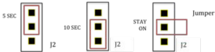
Receiver Alert Timer Duration Jumper Settings (Deluxe LR and Deluxe ELR Receivers only)
